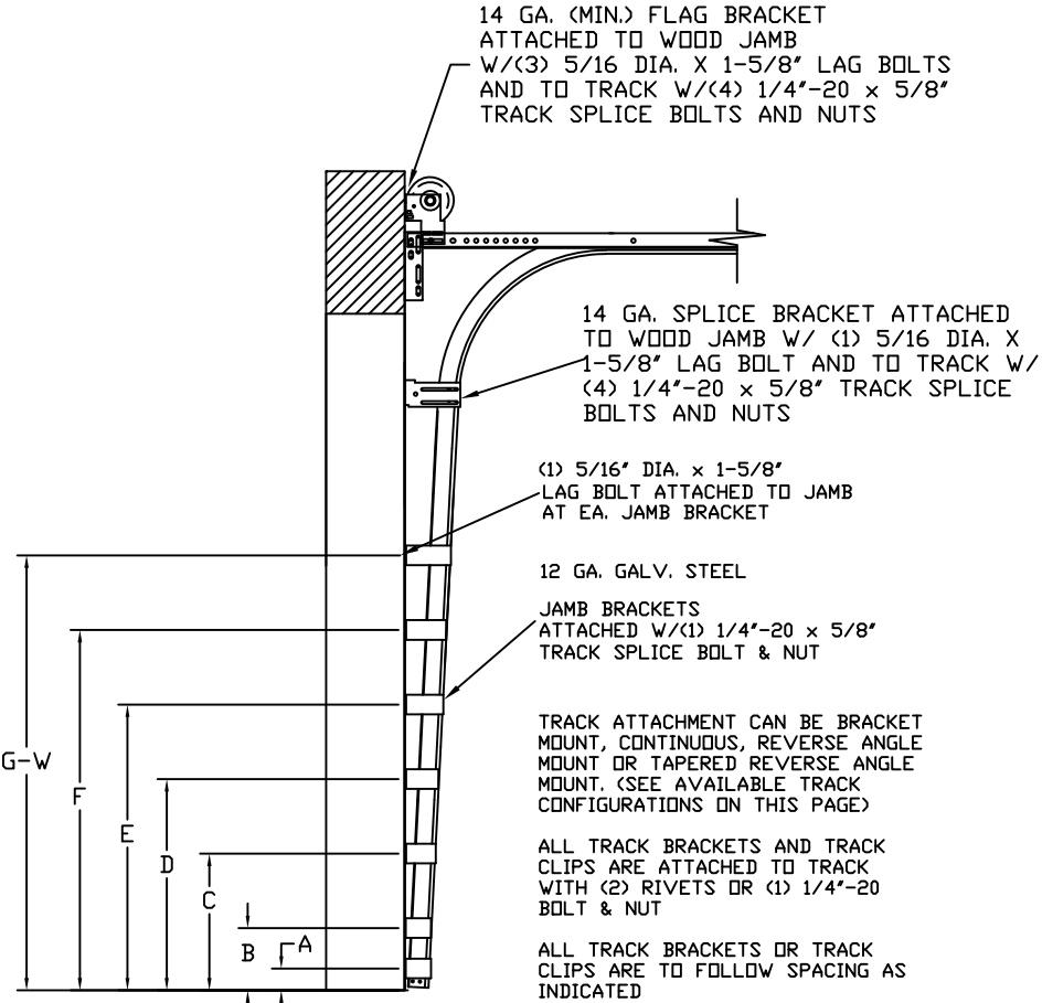
TRACK CONFIGURATION FOR UP TO 14' TALL DOORS
