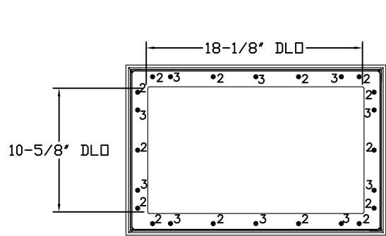
IMPACT GLAZING FASTENER DETAIL N.T.S. GLAZING MEETS ASTM E1300-04
